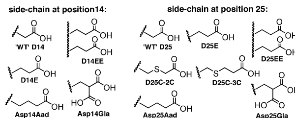
Figure 2. Side-chain structural variations at pHLP position 14 and 25. WT, D14E, and D25E are previously known. [10b,19]
